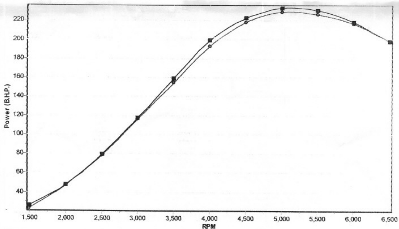
Power (B.H.P.)
